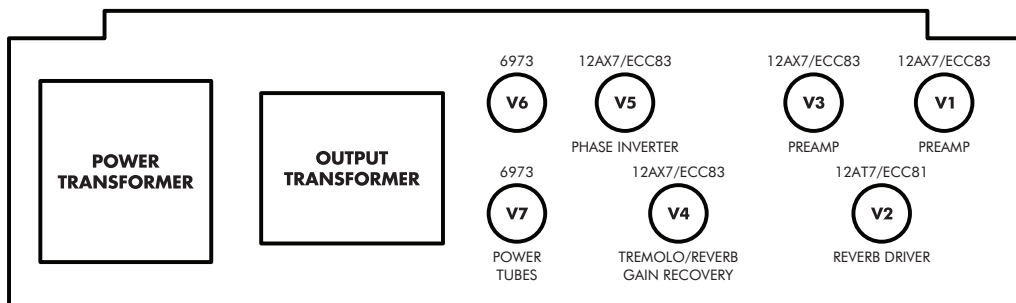
Black Magick Reverb Tube Layout:
